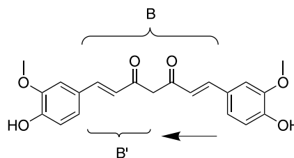
Figure 3. Proposed modification of curcumin's β-diketone linker region.
