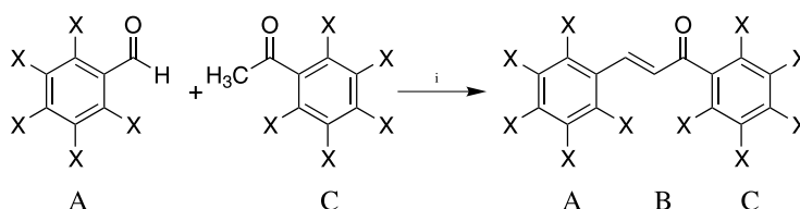
Scheme 1. Generalized synthetic scheme for the preparation of enone derivatives. Reagents and conditions: (i) 10–40% KOH, EtOH, 5–10 °C. Let stir ~4 h at room temperature. X = H, Cl, F, OCH 3 , CF 3 , OH, NH 2 , CH 3 , CH(CH 3 ) 2 , NO 2 , phenyl, OBn, and CH 2 COOH; A and C ring systems = benzene, 1-naphthalene, 2-naphthalene, 2-pyridine, 3-pyridine, 5-benzo[1,3]dioxole, 2-furan, 2-pyrrole, and 9-anthracene.
