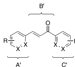
Figure 4. Generalized substitution patterns of the aromatic enone analogs investigated. R = Cl, F, CH 3 , NO 2 , isopropyl, OBn, phenyl, OCH 3 , and OH; X = C, N; A' and C' = benzene, pyridine, furan, pyrrole, naphthalene, anthracene, biphenyl, and benzo[1,3]dioxole.
